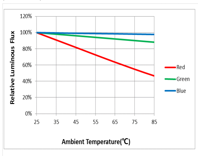
Fig 5. Ambient Temperature vs. Relative Luminous flux (IF=150mA)
