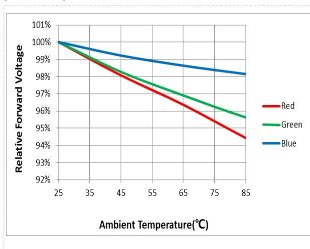
Fig 6. Ambient Temperature vs. Relative Forward Voltage (IF=150mA)
