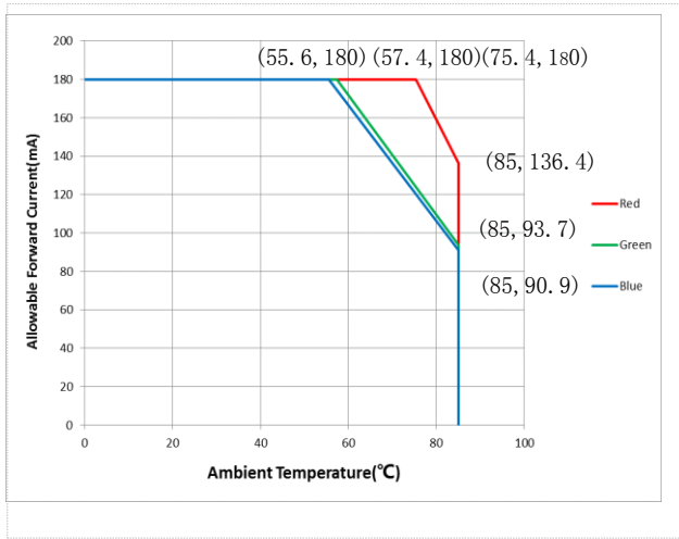
Fig 7. Ambient Temperature vs.Maximum Forward
