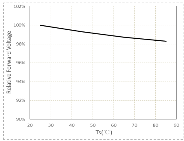
Fig 6. Surface Temperature vs. Relative Forward Voltage (IF=100mA)
